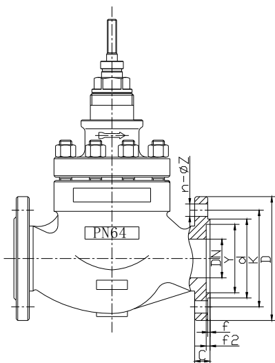
PN64 Valve Body End Flange Connection
