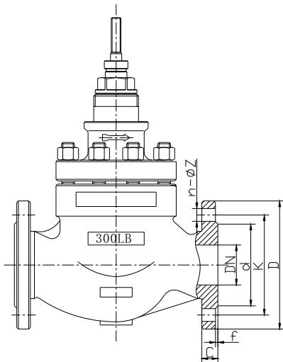
300LB Valve Body End Flange Connection
