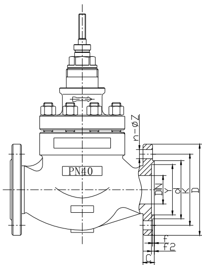
PN40 Valve Body End Flange Connection
