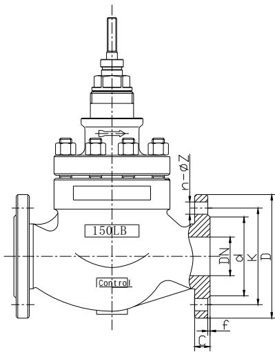
150LB Valve Body End Flange Connection
