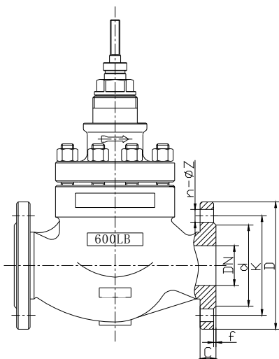
600LB Valve Body End Flange Connection
