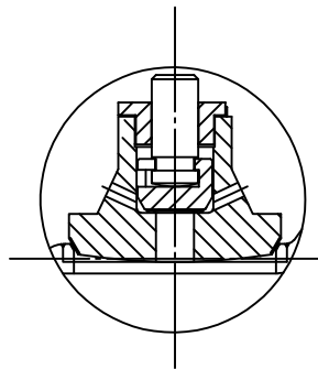
NPS >10 Completed with double disc
