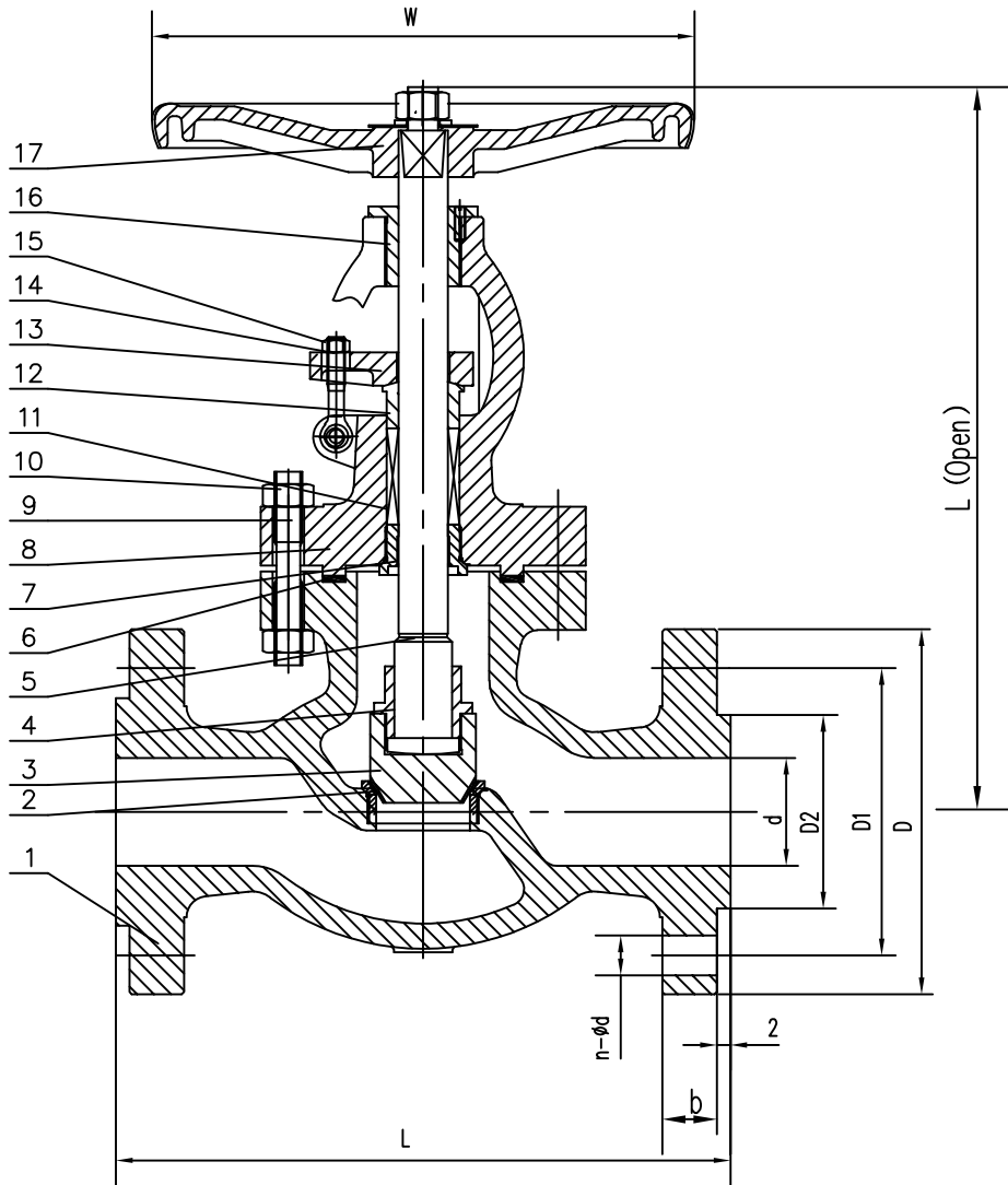
NPS >10 Completed with double disc
