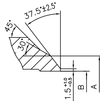
Butt-Weld End Amplification
