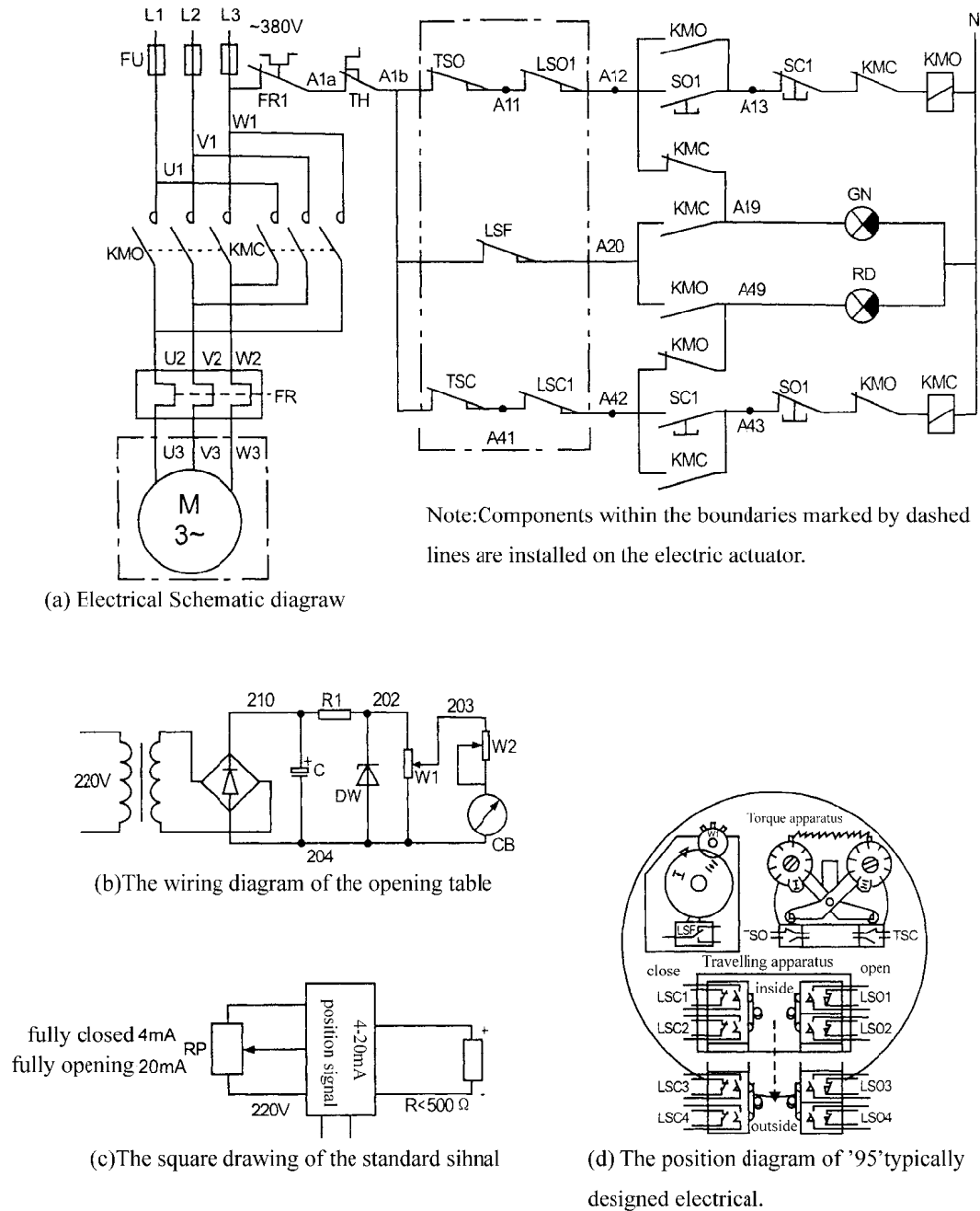
Picture 9: The electrical schematic diagram of DZW, DZ Boutdoor type.
